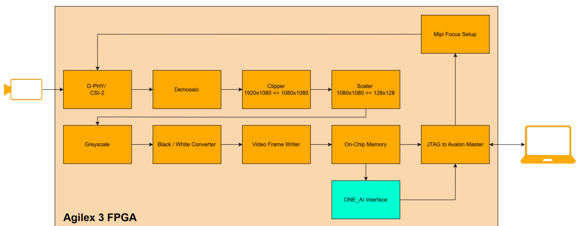
Figure 1: Block design of the AI on Agilex 3 FPGA system
